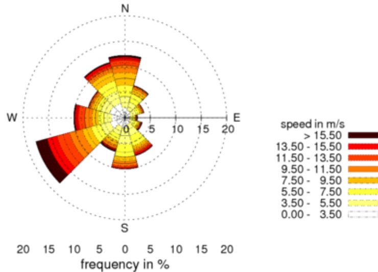
Figure 2. Wind rose for the dummy climatology 2022 (to be used in the 2022 Championship)
